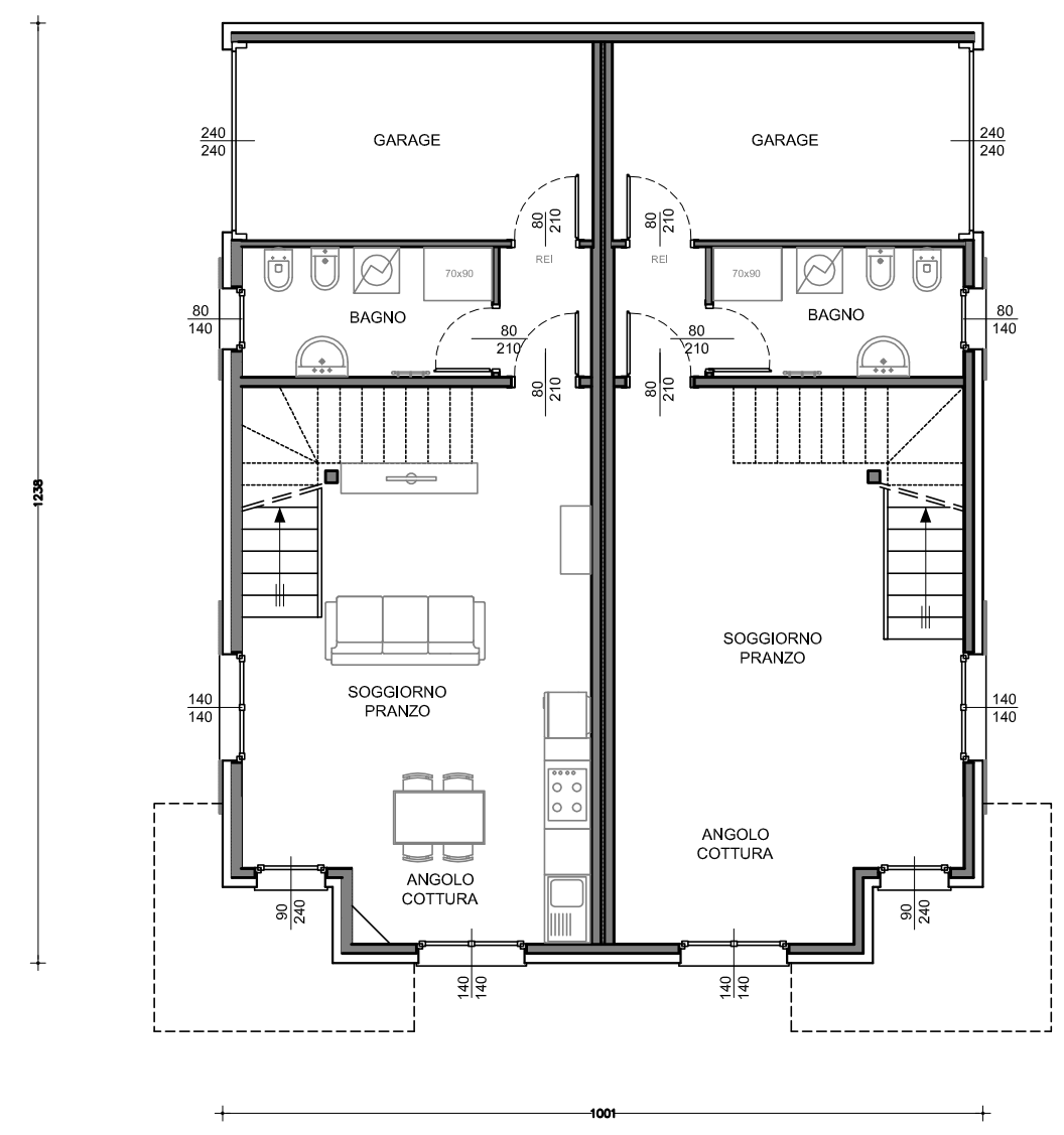
PIANO TERRA
